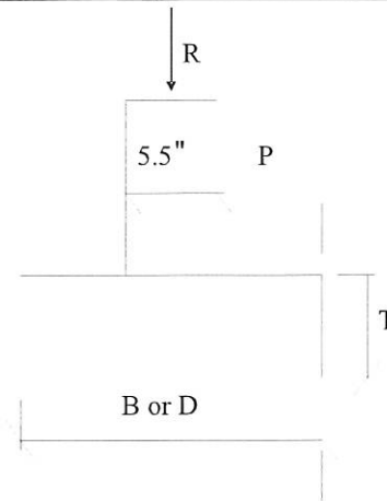
Figure C12. Footing Dimensions and Variables.
